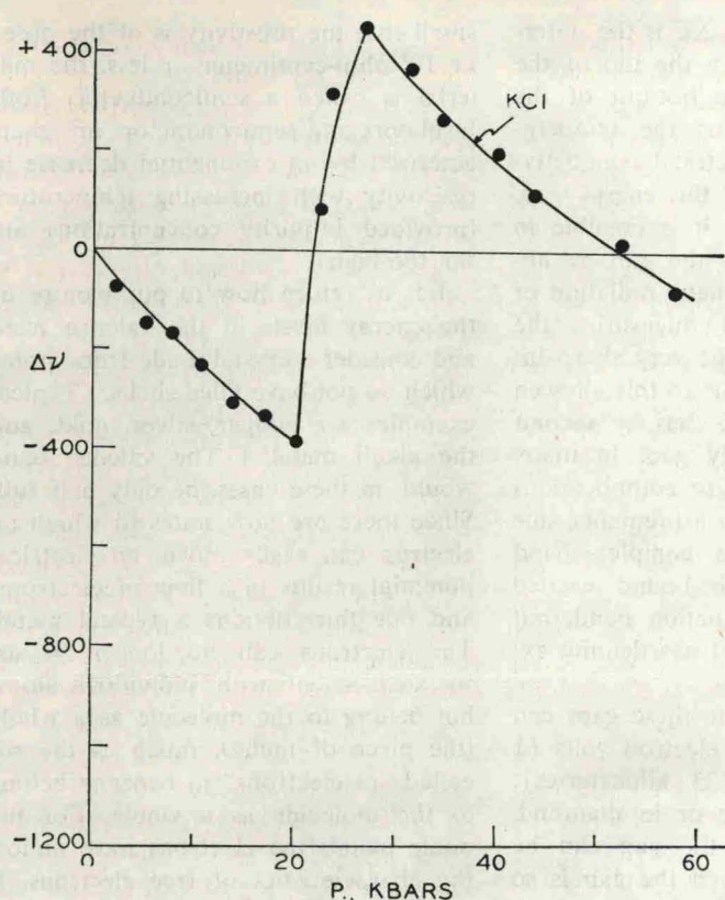
Fig. 2 (left). \Delta V plotted against pressure for potassium chloride with \text{TI}^+ . Fig. 3 (right). \Delta V plotted against pressure for \text{TI}^+ in alkali halides.
