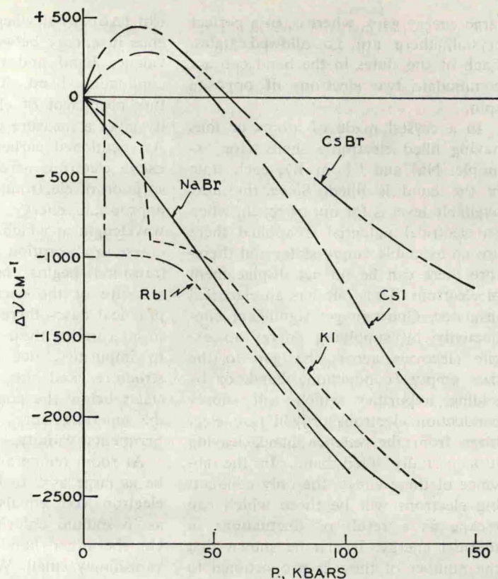
Fig. 2 (left). \Delta V plotted against pressure for potassium chloride with \text{TI}^+ . Fig. 3 (right). \Delta V plotted against pressure for \text{TI}^+ in alkali halides.
